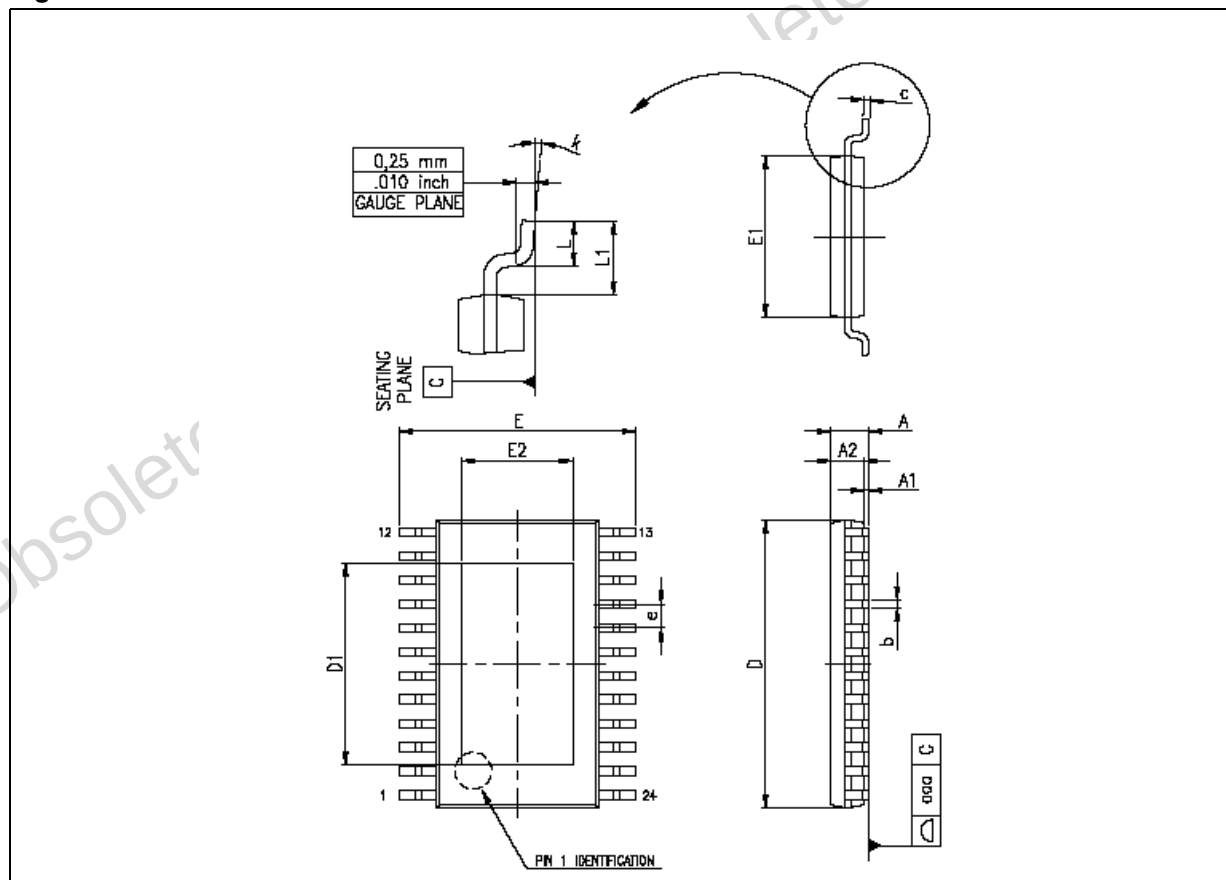
Figure 22. TSSOP24 dimensions
