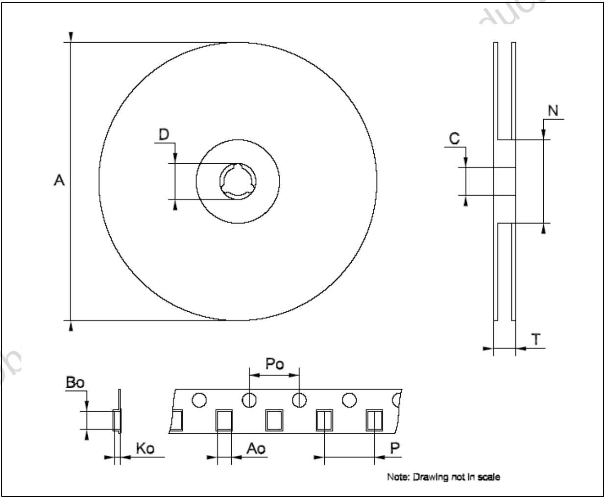
Figure 21. Reel dimensions
