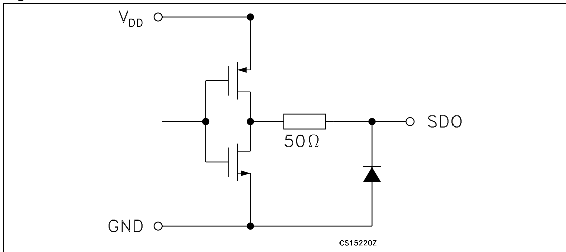
Figure 5. SDO terminal
