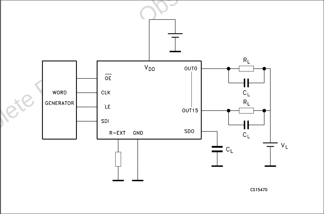
Figure 12. AC characteristics
